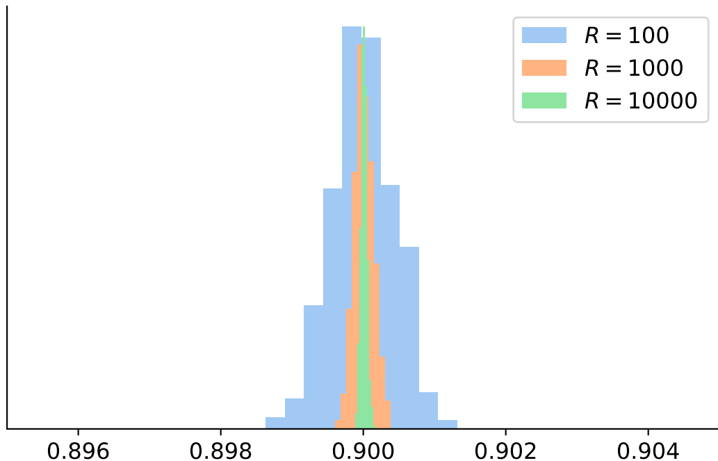
Distribution of \bar{C} with n = 10000 , n_{\text{val}} = 10000
